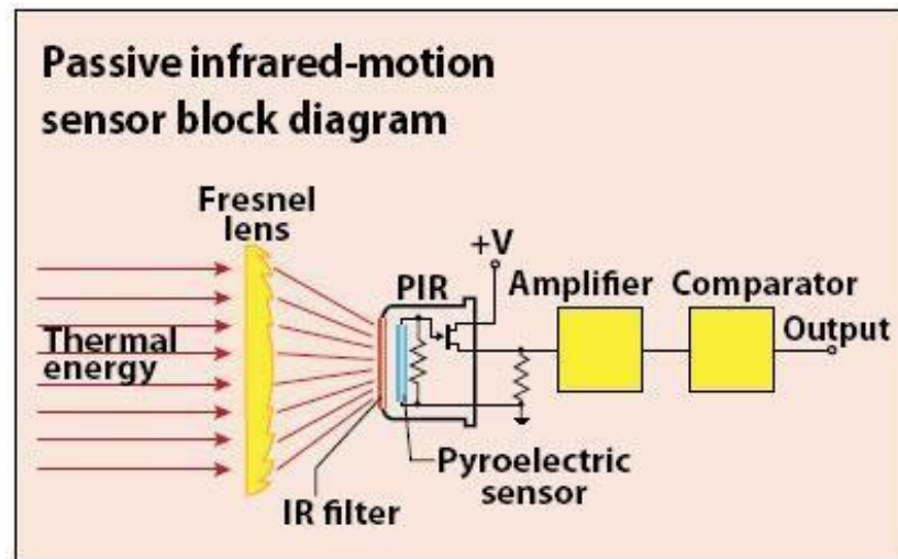
Gambar 2.6 Diagram Blok Sensor PIR ( Passive Infra Red )
