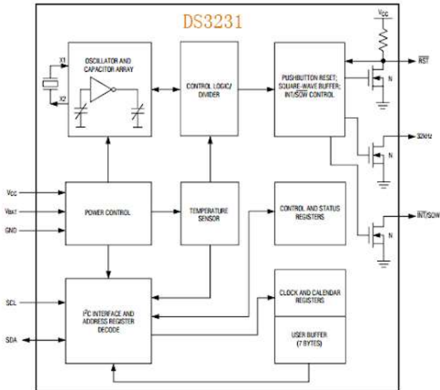
Gambar 2.8 Blok Diagramm RTC DS3231
