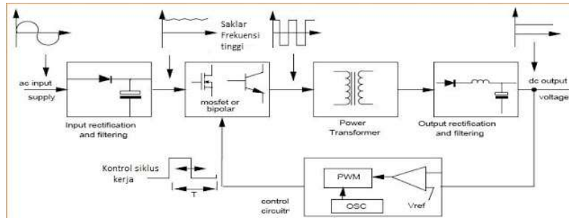
Gambar 2.2 Block Diagram Regulated Power Supply
