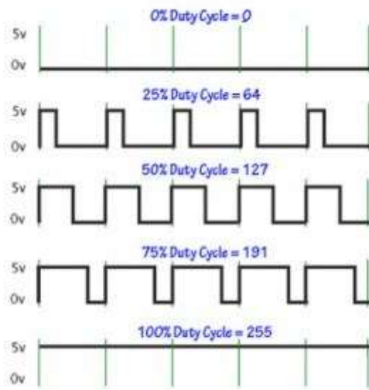
Gambar 2.11 Pulsa PWM
