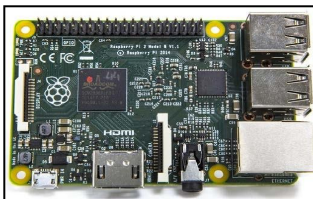
Gambar 2.4. Raspberry Pi 2 Model B
