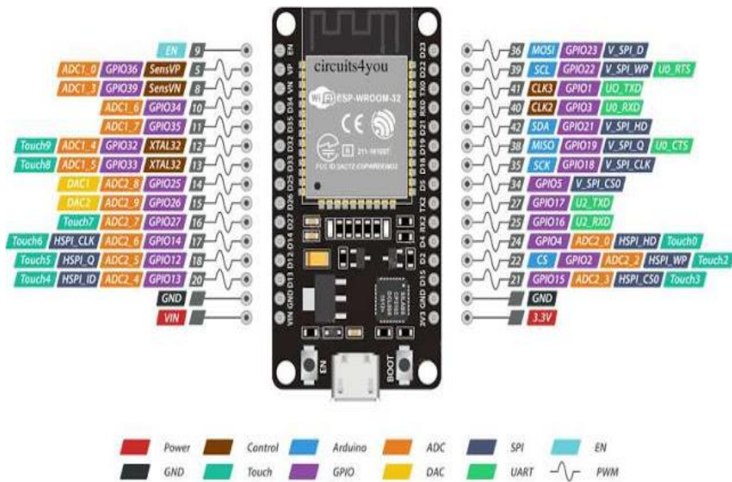
ESP32 Dev. Board Pinout
