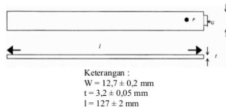
Gambar 2. Spesimen Uji (ASTM D995-08)
