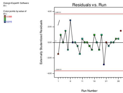
Figure 3 Residual vs Run
