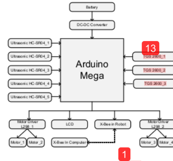
Fig. 3. Block Diagram of Odor Localization Robot
