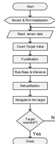
Fig. 4. Flowchart of Fuzzy algorithm
