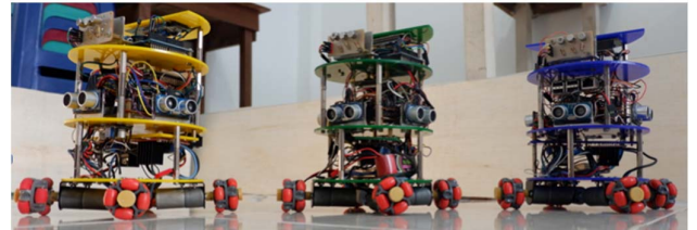
Fig. 1. 3 Agents used as swarm robot, Cyborg-G11, Cyborg-G12, and Cyborg-G13
