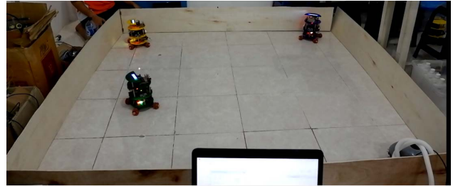
Fig. 7. Swarm robots' position in the first 30 second.
