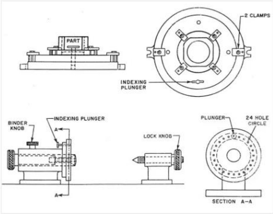
Gambar 2. 14 fixture Indexing
