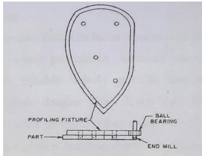
Gambar 2. 16 Fixture profil
