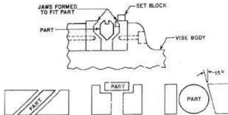
Gambar 2. 12 Fixture Vise-jaw
