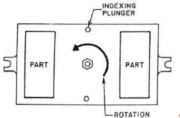
Gambar 2. 15 Fixture duplex
