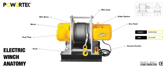
Gambar 2.9 komponen Electric Winch (Sumber : https://otopedia.com/berita/winch/ )
