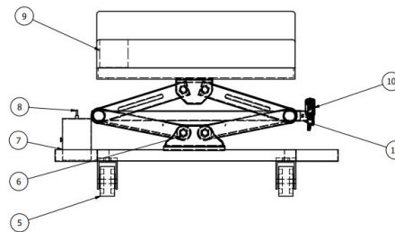
Gambar 2.7 Mechanic Creeper Semi Elektrik Tampak Kiri [10]
