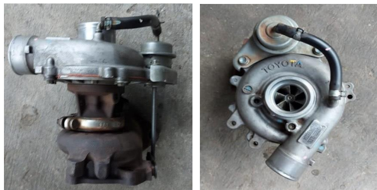
Gambar 2.6 Turbocharger [8]
