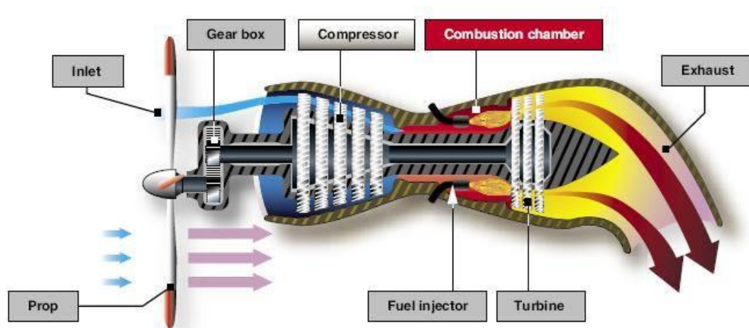
Gambar 2.4 Turboprop [4]
