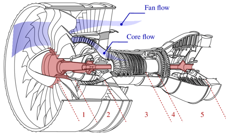
Gambar 2.5 Turbofan [5]
