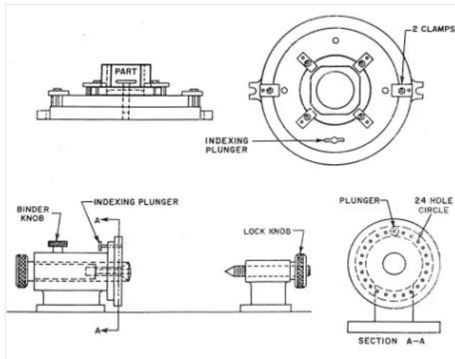
Gambar 2. 14 fixture Indexing
