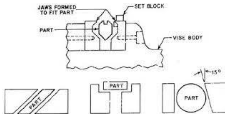
Gambar 2. 12 Fixture Vise-jaw
