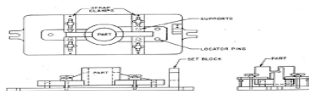
Gambar 2. 9 fixture pelat
