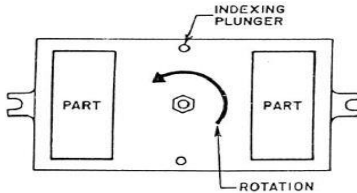
Gambar 2. 15 Fixture duplex
