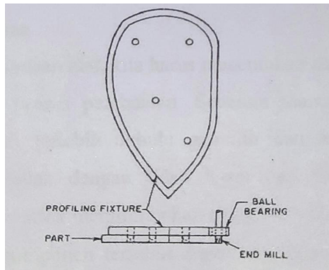
Gambar 2. 16 Fixture profil
