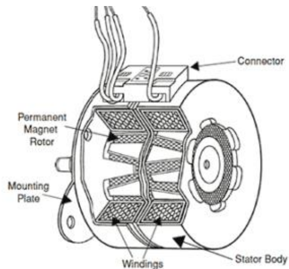
Gambar 2.4 Motor Stepper Permanent Magnet [2]
