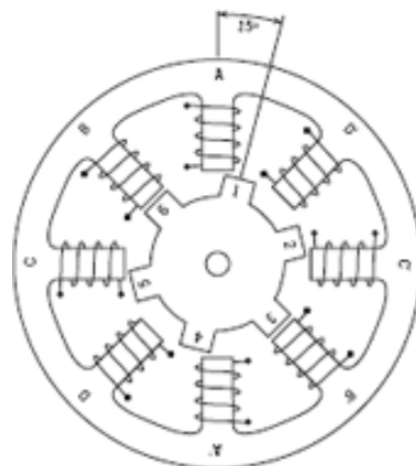
Gambar 2.6 Motor Stepper Variable Reluctance [2]
