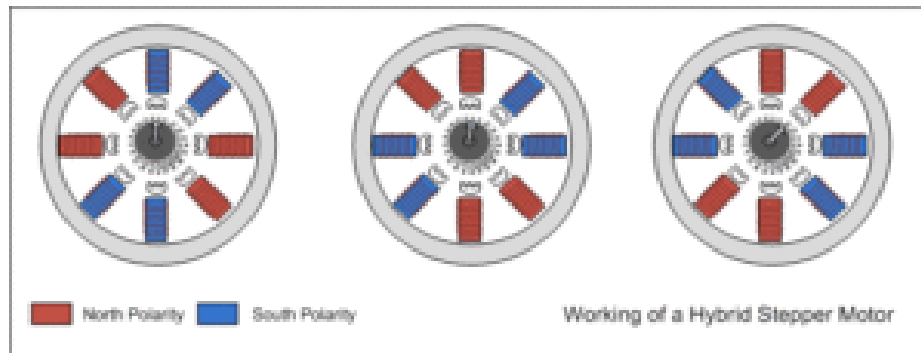
Gambar 2.5 Motor Stepper Hybrid [2]
