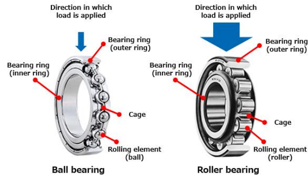
Gambar 2.30 Ball Bearing dan Roll Bearing [12]
