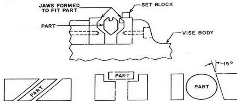
Gambar 2.23 Fixture vise-jaw [23]
