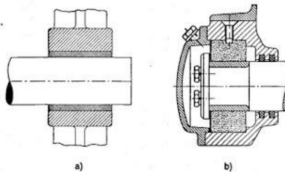
Gambar 2.29 a. Journal Bearing , b. Rolling Bearing [12]
