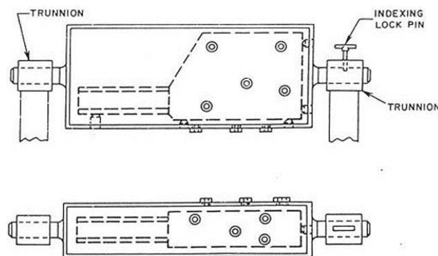
Gambar 2.17 Jig Trunnion [23]
