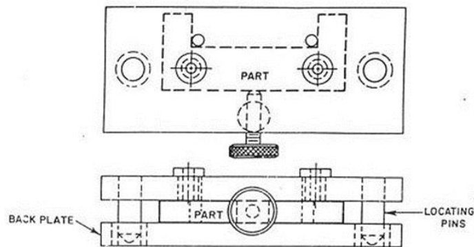
Gambar 2.10 Jig Sandwich [23]
