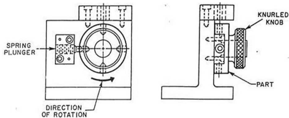
Gambar 2.16 Jig Indexing [20]
