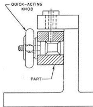
Gambar 2.11 Jig Angel Plate [23]
