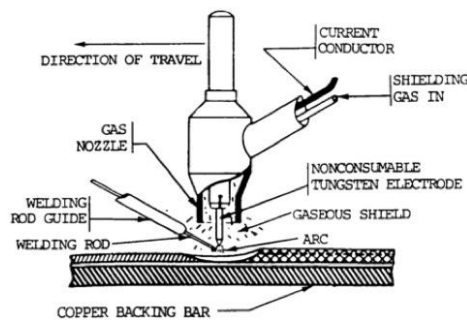
Gas tungsten arc (TIG) welding (GTAW).
