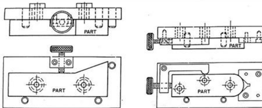
Gambar 2.9 Jig Plate [23]
