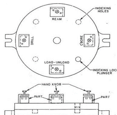
Gambar 2.19 Jig Multistation [23]
