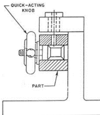
Gambar 2.12 Jig Angel Plate [5]
