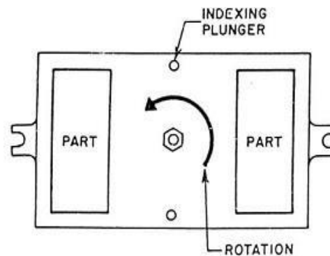
Gambar 2.27 Fixture duplex [4]
