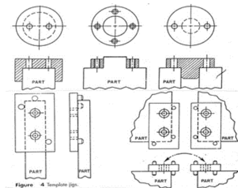
Gambar 2.9 Jig Template [5]
