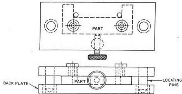
Gambar 2.11 Jig Sandwich [5]
