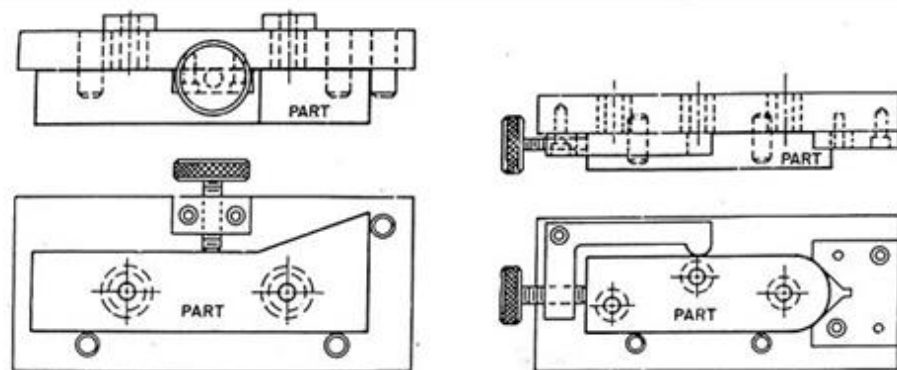
Gambar 2.10 Jig Plate [5]
