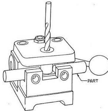
Gambar 2.19 Jig Pompa [5]
