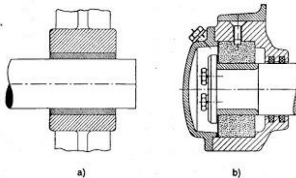
Gambar 2.30 a. dry sliding, b. Sintered bearing [8]
