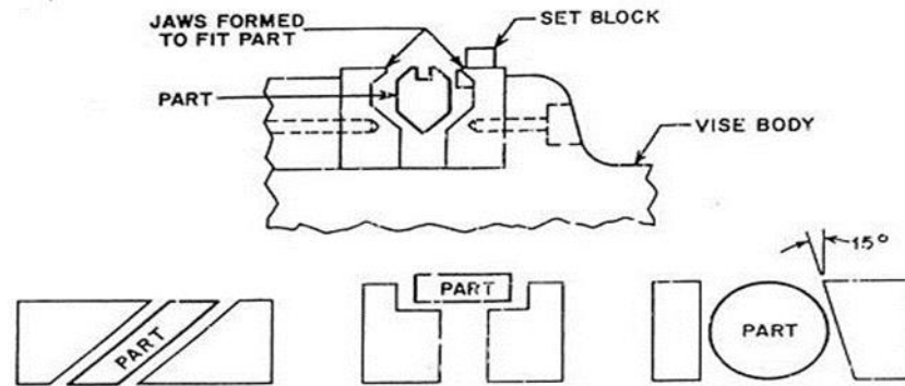
Gambar 2.24 Fixture vise-jaw [4]
