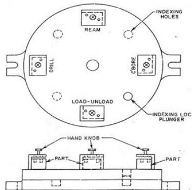
Gambar 2.20 Jig Multistation [5]
