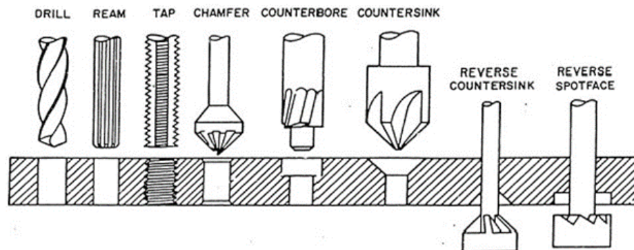
Gambar 2.8 Operasi umum Jig Gurdi [5]
