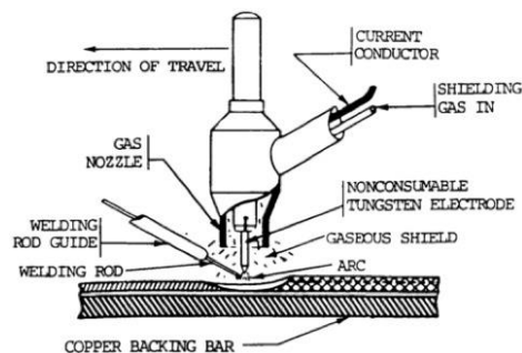
Gas tungsten arc (TIG) welding (GTAW).
