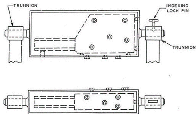
Gambar 2.18 Jig Trunnion [5]
