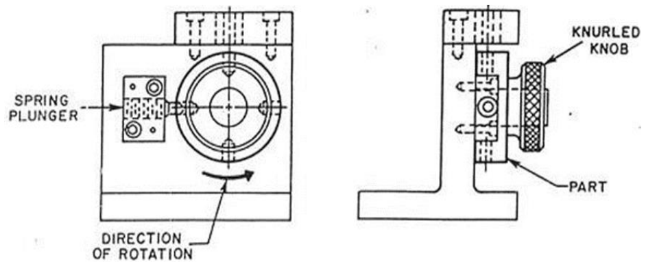
Gambar 2.17 Jig Indexing [5]
