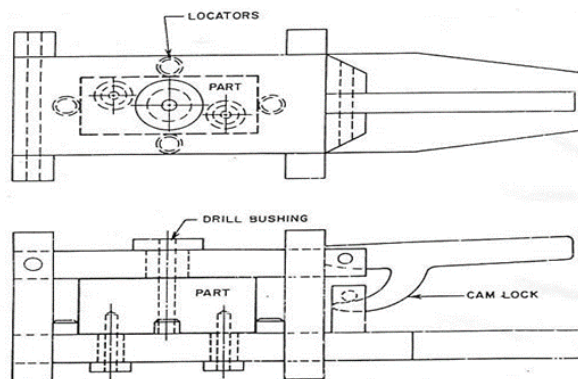
Gambar 2.16 Jig Leaf [5]
