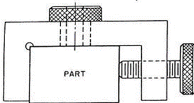
Gambar 2.15 Jig Channel [5]
