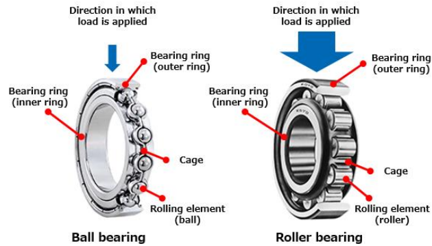
Gambar 2.31 Ball Bearing dan Roll Bearing [8]
