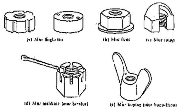
Gambar 2.34 Macam-macam mur [8]
