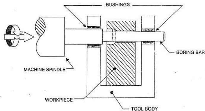
Gambar 2.7 Jig Bor [5]
