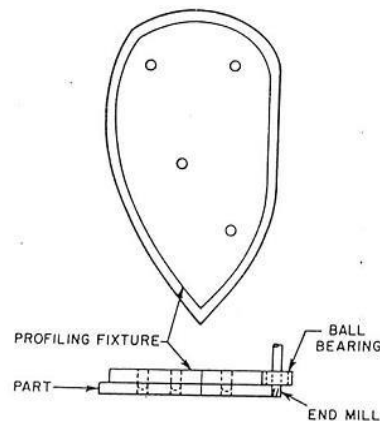
Gambar 2.28 Fixture profil [4]
