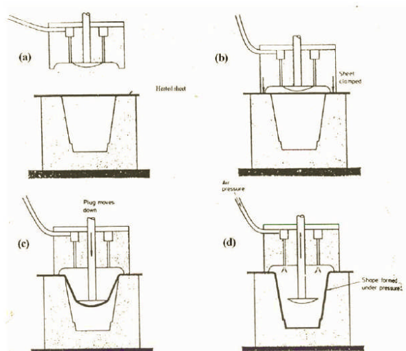
Gambar 2.1. Pressure Forming Process
