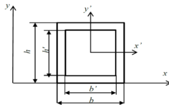
Gambar 2.18 Penampang Hollow (Sumber: Widodo. 2009)
