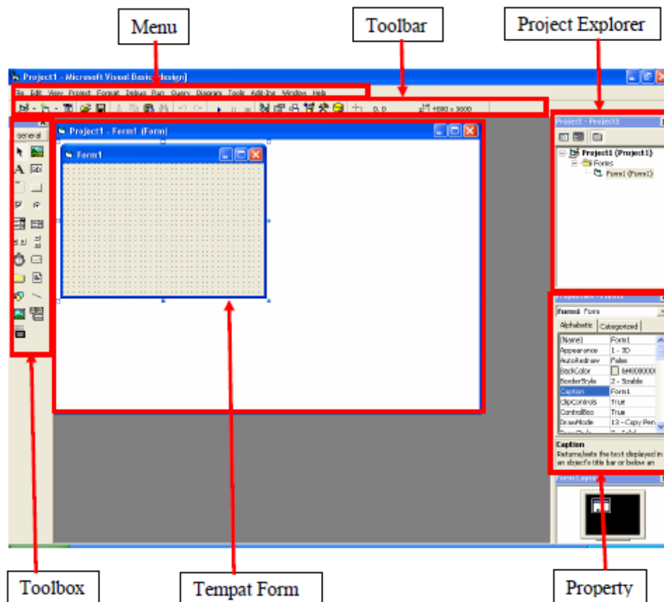
Gambar 2.24. Interface antar muka Visual Basic 6.0
