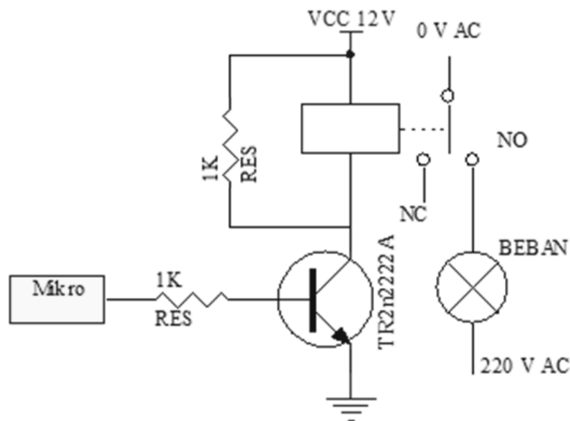
Gambar 2.6 Rangkaian Driver Relay ( Sumber : PCcontrol.wordpress.com)
