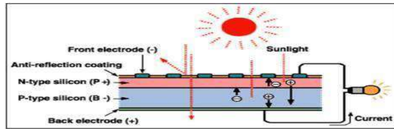
Gambar 2.7 Gambar Efek Photovoltaic
