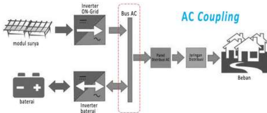
Gambar 2.2 Gambar Sistem PLTS off-grid tipe AC Coupling
