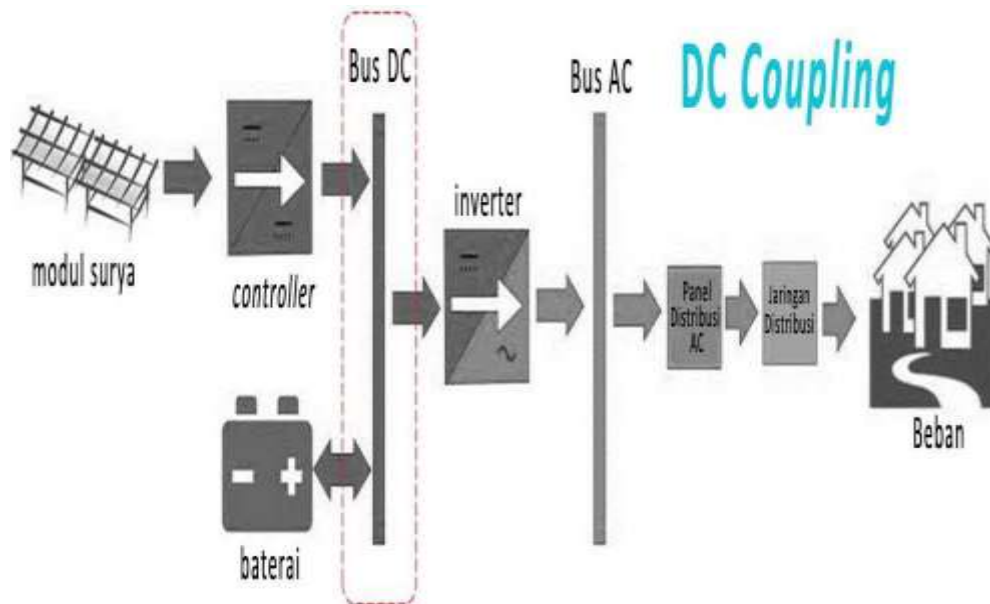
Gambar 2.1 Gambar Sistem PLTS off-grid tipe DC Coupling
