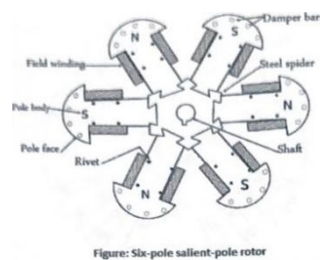
Gambar 2.5 Rotor Kutub Menonjol 4
