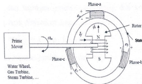
Gambar 2.1 Prinsip Kerja Generator Sinkron
