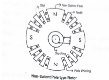
Gambar 2.6 Rotor Kutub Silinder 5
