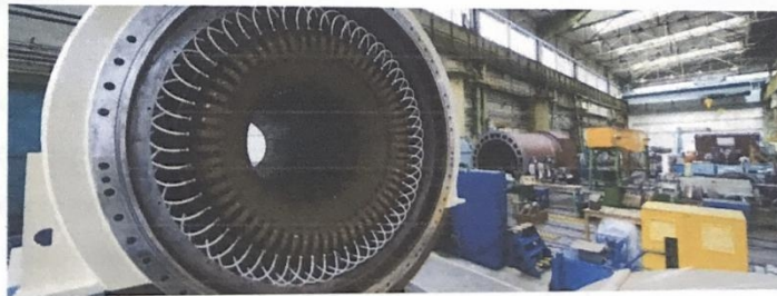
Gambar 2.2 Stator 1
