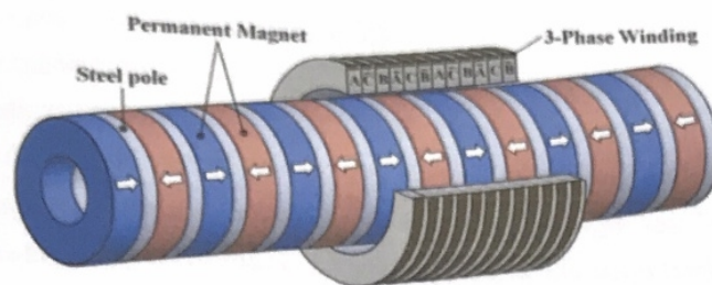
Gambar 2.19 Permanen Magnet Generator 11
