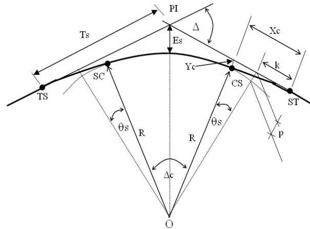
Gambar 2.15 Tikungan Spiral – Circle – Spiral (SCS)
