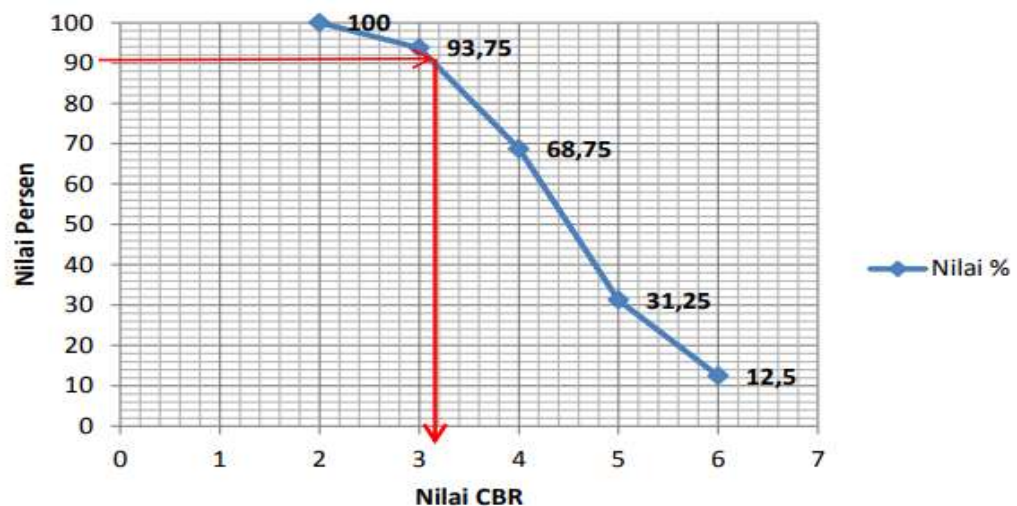
Gambar 2.29 CBR Segmen
