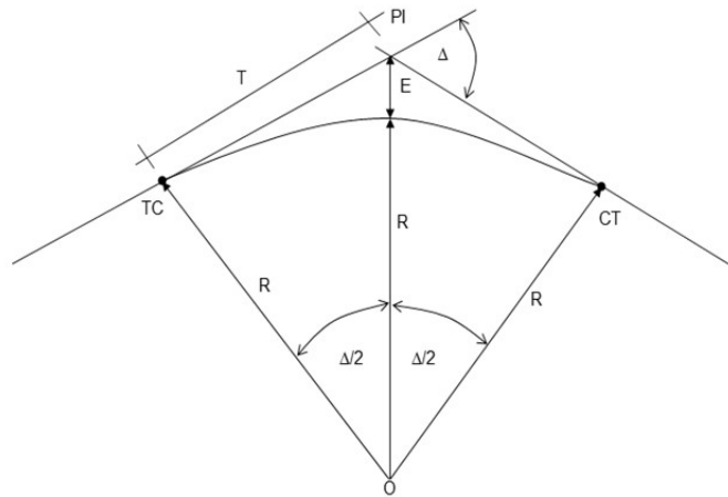
Gambar 2.14 Tikungan Full Circle (FC)
