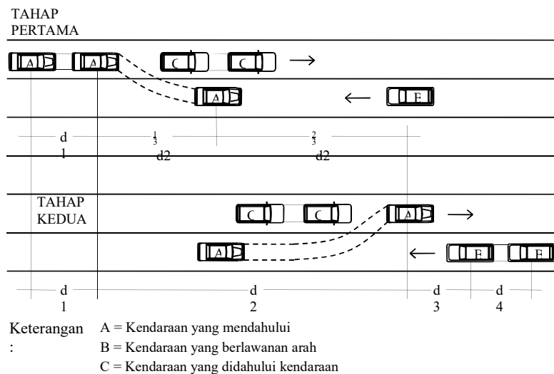
Gambar 2.20 Proses Gerakan Mendahului (2/2 TB)
