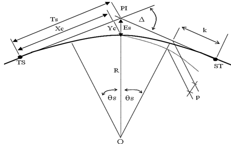
Gambar 2.13 Tikungan Spiral – Spiral (SS)
