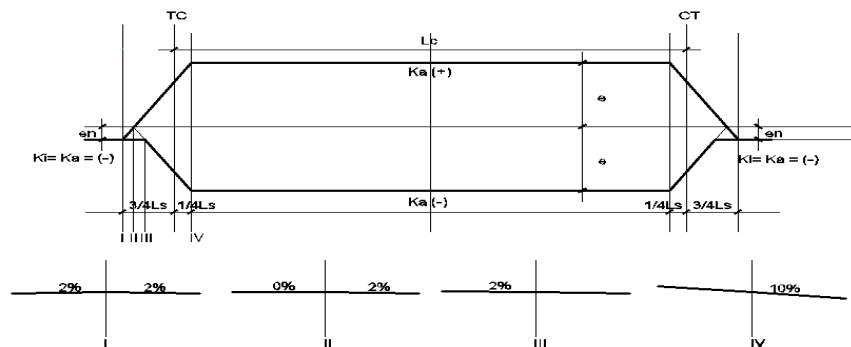
Gambar 2.15 Diagram Superelevasi Full Circle
