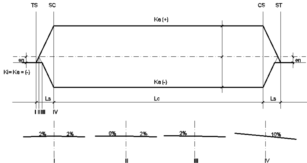
Gambar 2.16 Diagram Superelevasi Spiral – Circle - Spiral
