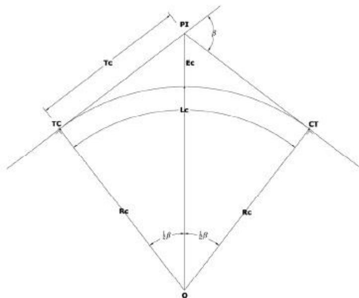
Gambar 2.17 Tikungan Full Circle
