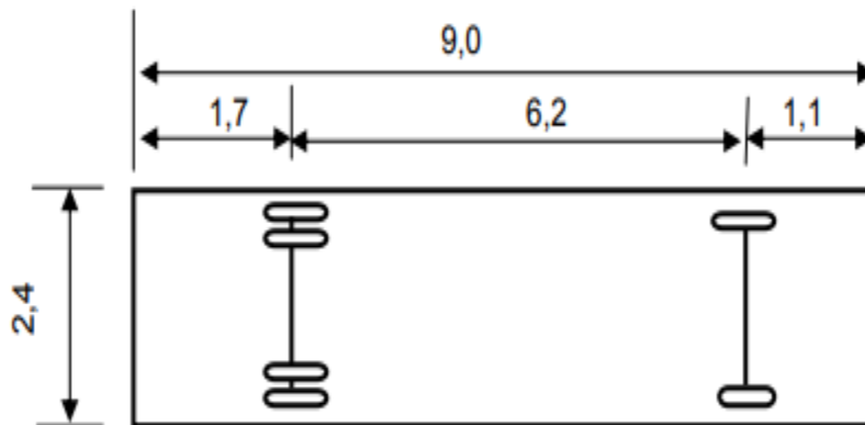
Gambar 2.8 Kendaraan Truk As Tunggal (SU)
