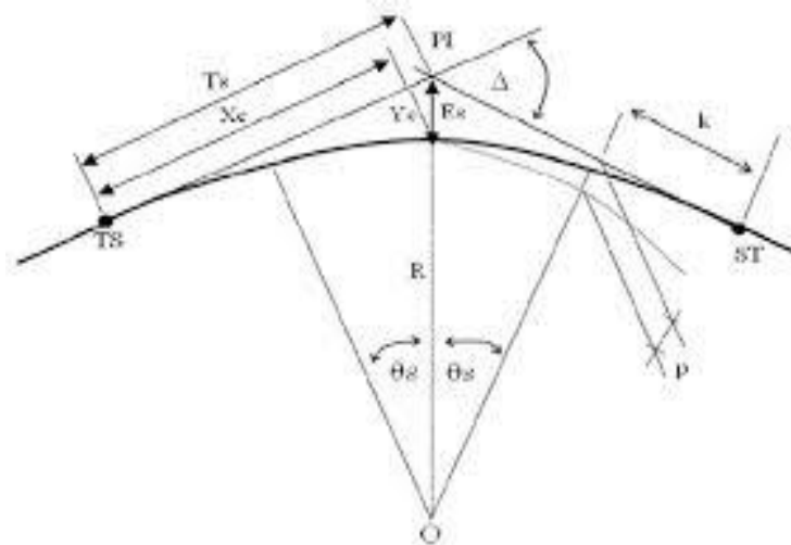
Gambar 2.19 Tikungan Spiral – Spiral
