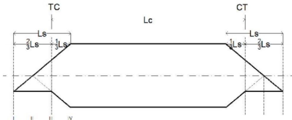
Gambar 2.20 Diagram Pencapaian Superelevasi Full Circle
