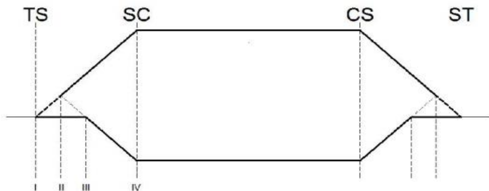
Gambar 2.21 Diagram Pencapaian Superelevasi Spiral – Circle – Spiral
