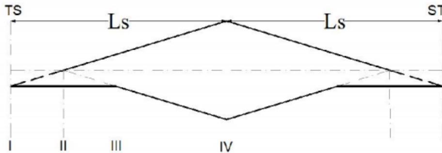
Gambar 2.22 Diagram Pencapaian Superelevasi Spiral – Spiral
