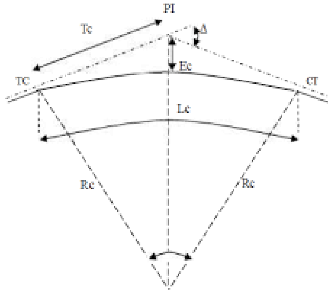
Gambar 2.18 Tikungan Spiral – Circle – Spiral
