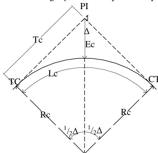
Gambar 2.8 Lengkung Full Circle
