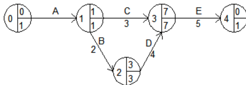
Gambar 2.37 Sketsa Network Planning
