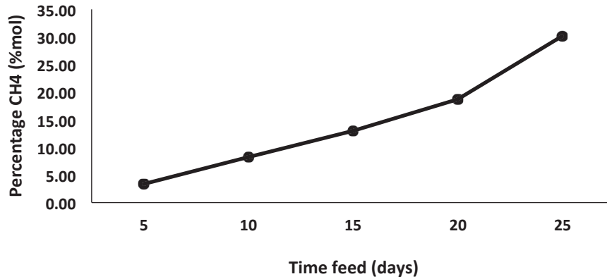
Figure 4. The Effect of Time on Five Days of Feed POME on CH 4 Production
