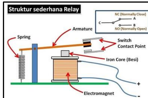
Gambar 2.7 Bagian-bagian Relay
