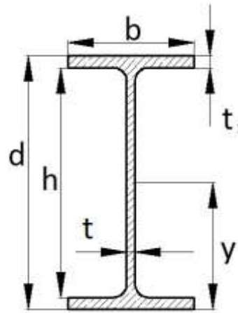
Gambar 2.24 Penampang WF-Beam (eprint 2012)
