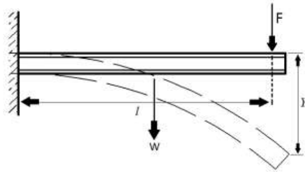
Gambar 2.25 Lenturan WF-Beam
