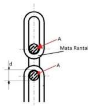
Gambar 2.17 Mata rantai lasan (Adoc.tips 2018)
