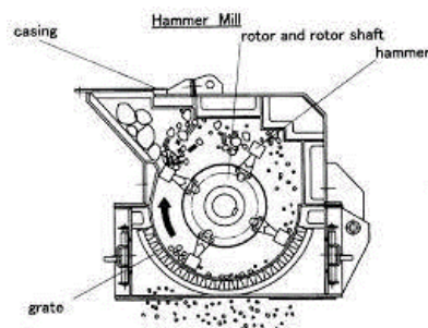
Gambar 2.3 Hummer Mill
