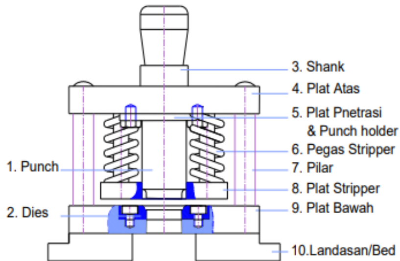
Gambar 2.1 Simple tool (Arifin Fatahul, 2010)
