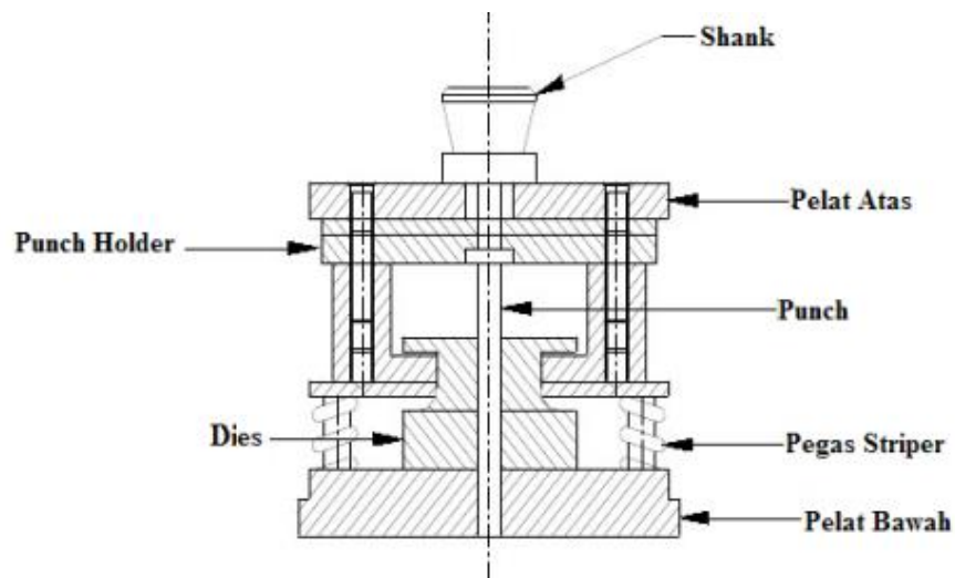
Gambar 2.2 Compound Tool (Arifin Fatahul, 2010)
