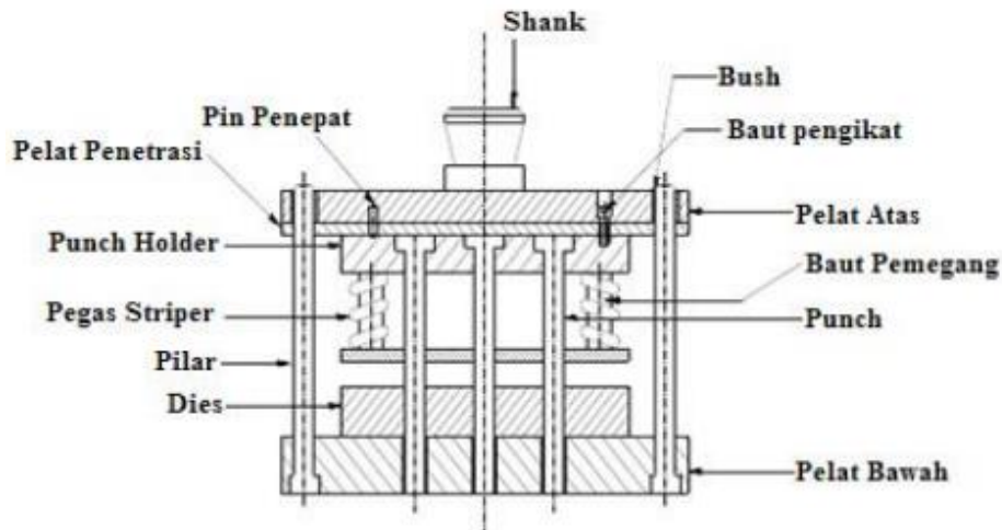
Gambar 2.3 Progressive Tool (Arifin Fatahul, 2010)
