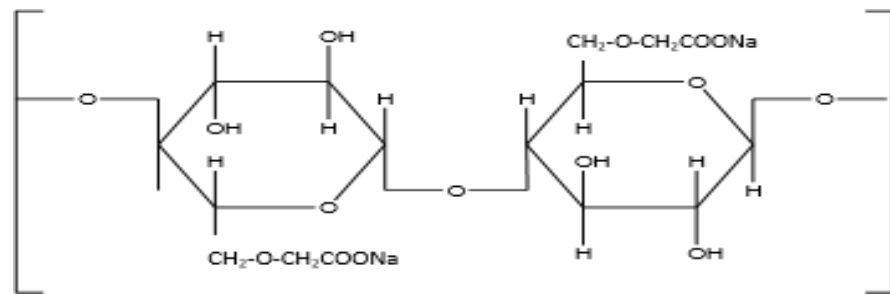
Gambar 2.14 Struktur CMC (Carboxymethyl Cellulose) (Kamal, 2010)
