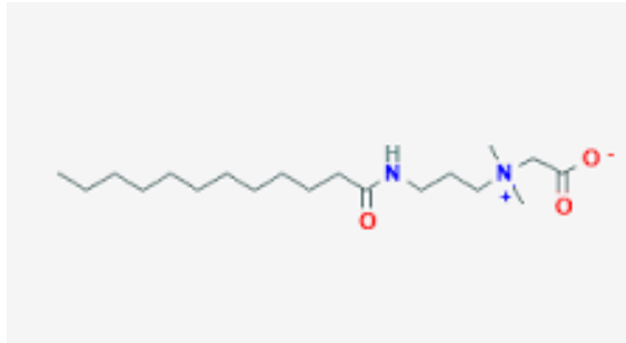
Gambar 2.10 Struktur Kimia Cocoamidopropyl Betaine ( Handbook of Pharmaceutical Excipients Fifth Edition , 2006)
