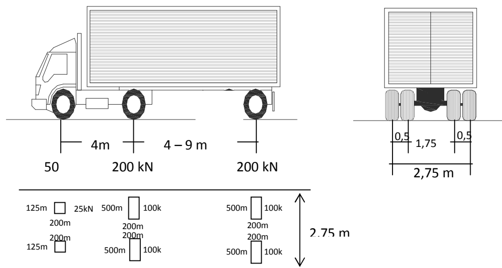
Gambar 2.5 Pembebanan truck “T” (500kN)
