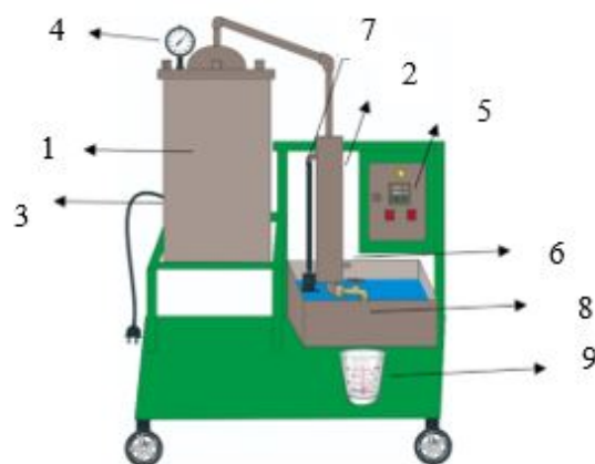
Figure 1. Thermal Catalytic Cracking Reactor
