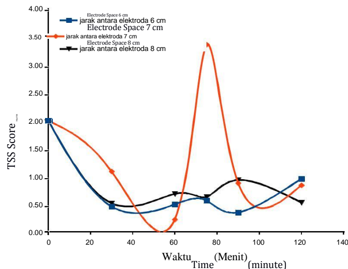
Figure 3. TSS value at each electrocoagulation time
