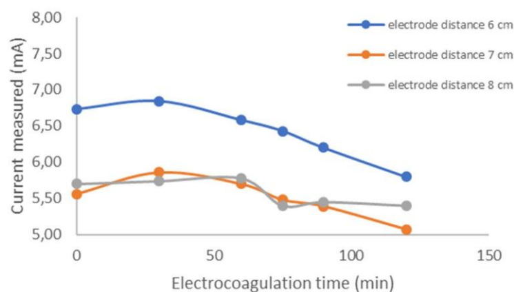
Figure 1. Current changing during electrocoagulation process
