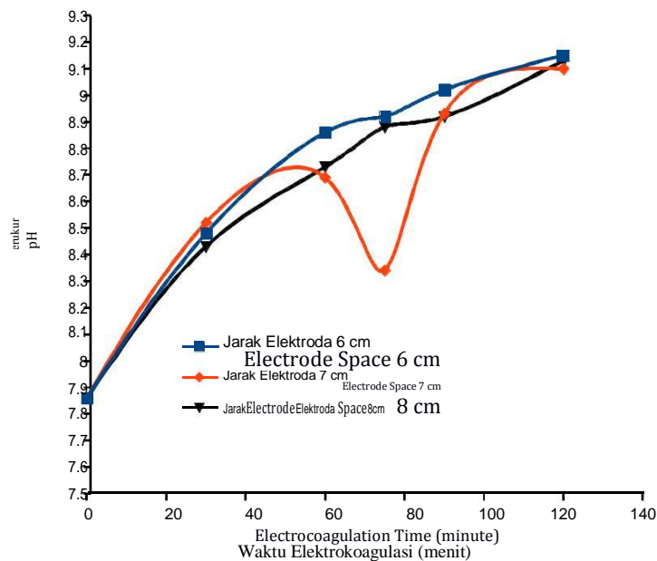
Figure 2. Value of pH at each electrocoagulation time
