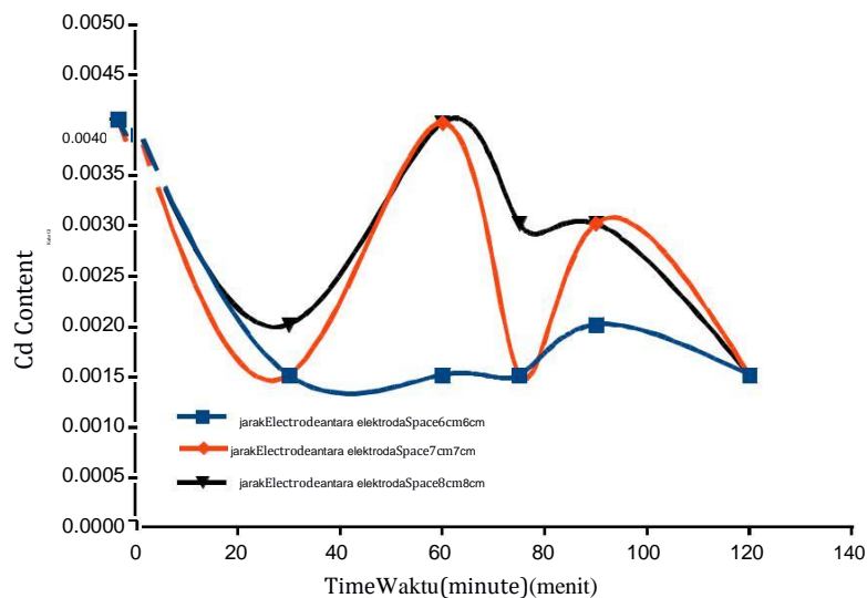
Figure 6. Cd content at each electrocoagulation time
