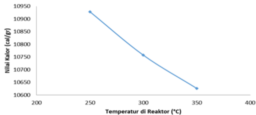
Figure 6. Effect of Temperature Variations on Heating Value
