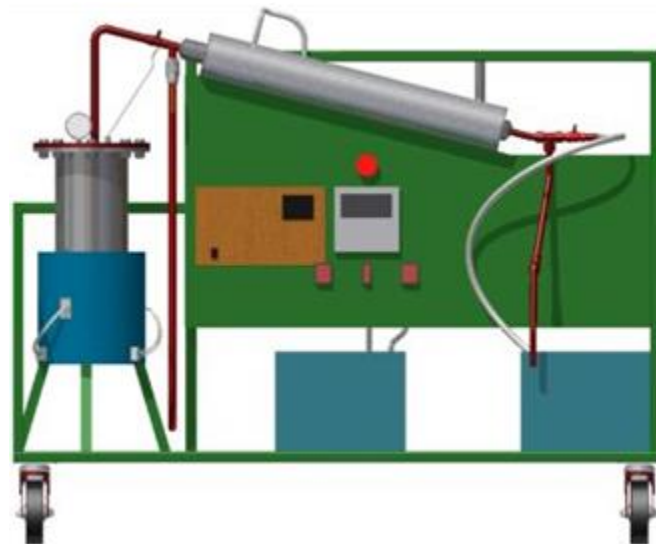
Figure 1. Pyrolysis Equipment Scheme
