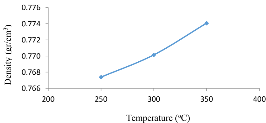
Figure 4. Effect of Temperature Variations on Density
