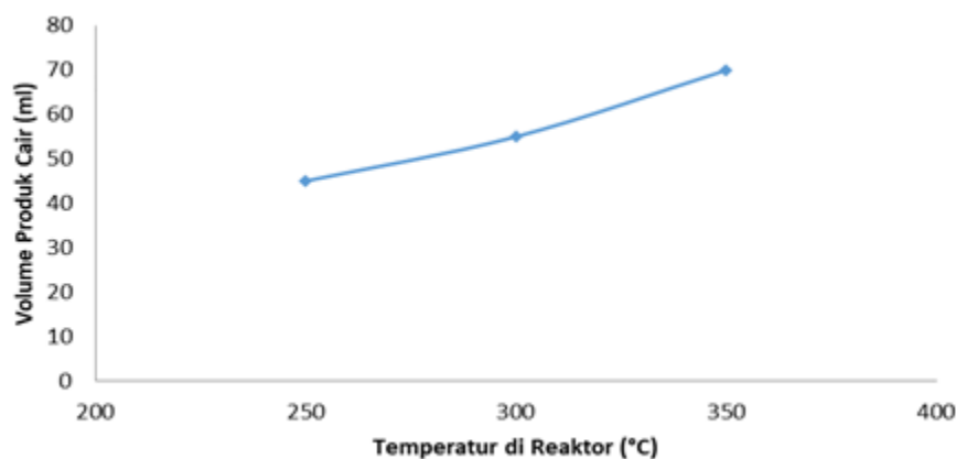
Figure 2. Effect of Temperature on Pyrolysis Liquid Product Volume
