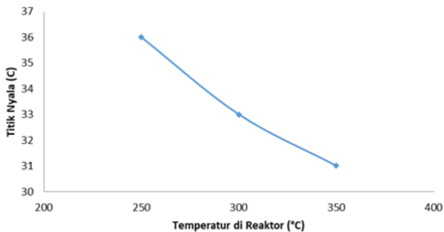
Figure 7. Effect of Temperature Variations on Flash Points
