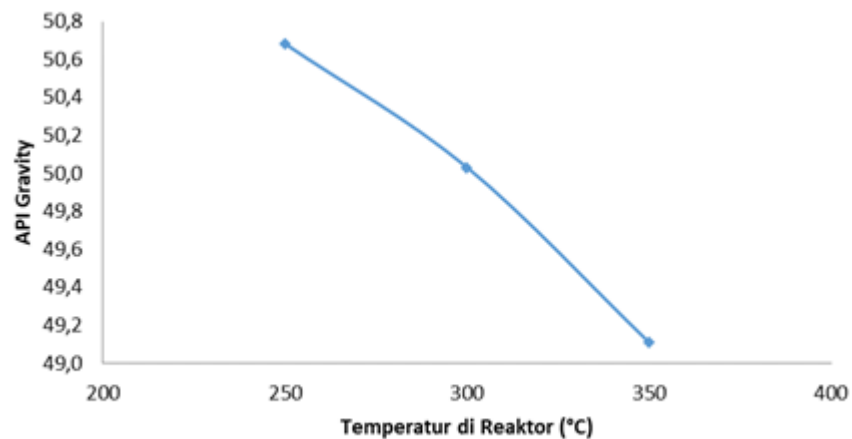
Figure 5. Effect of Temperature Variations on API Gravity
