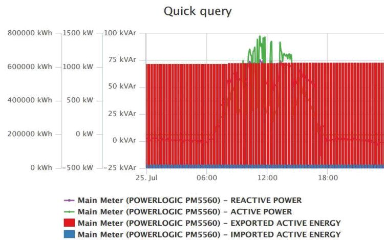
Figure 6. PV panels energy produced by Jakabaring Solar Power Plant on July 25, 2018.
