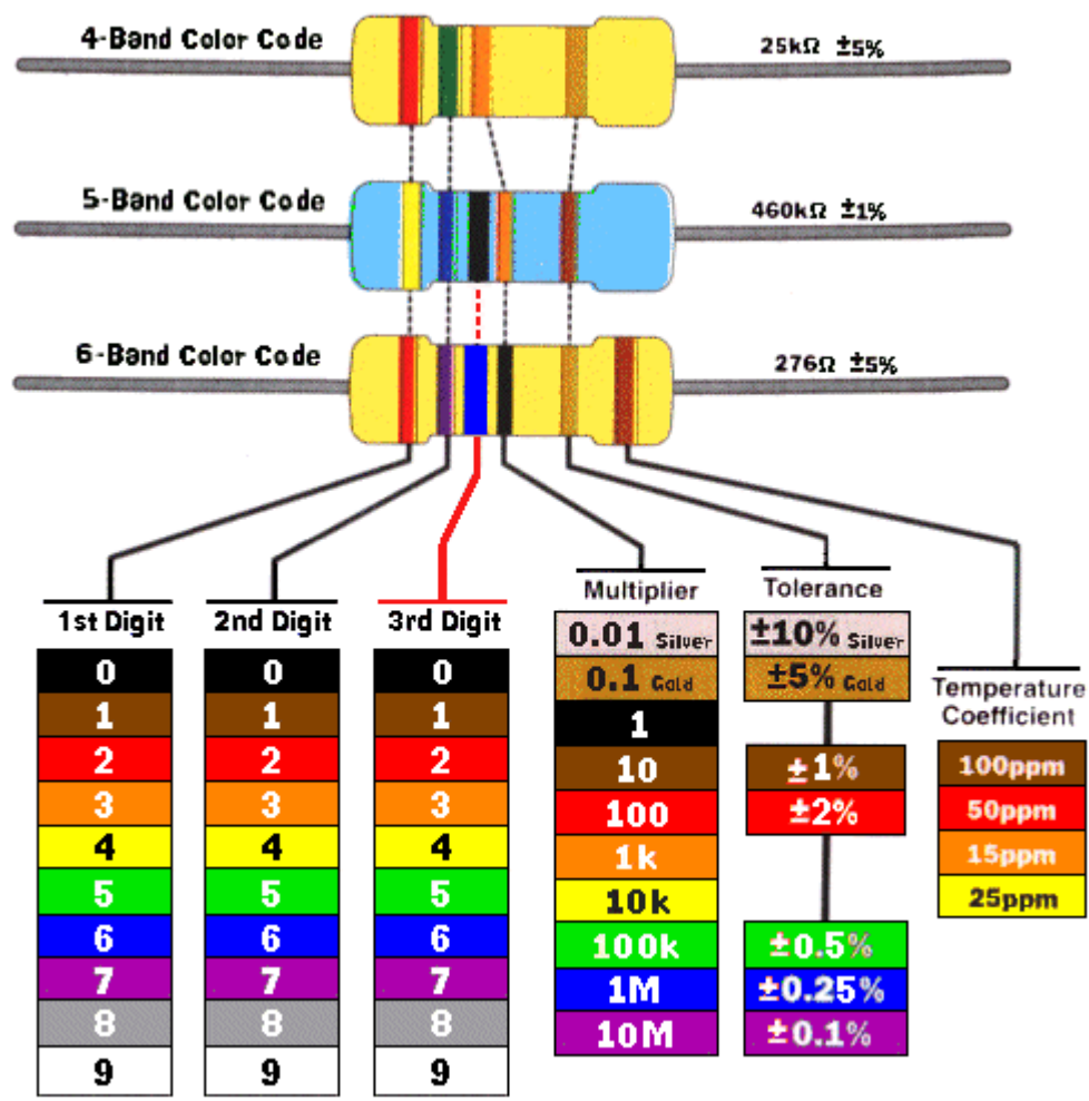
Gambar 2. 12 Resistor
