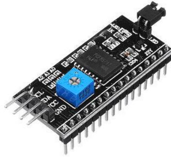
Gambar 2. 6 I2C
