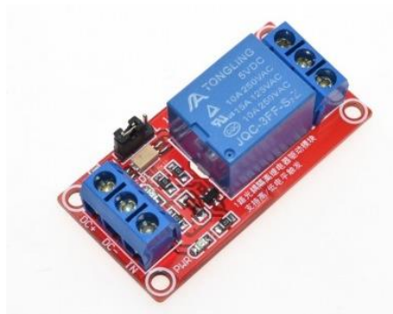
Gambar 2. 11 Relay 1 Channel
