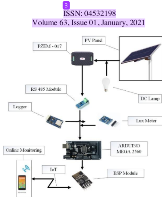
Figure 1. The proposed IoT monitoring system for a PV panel
