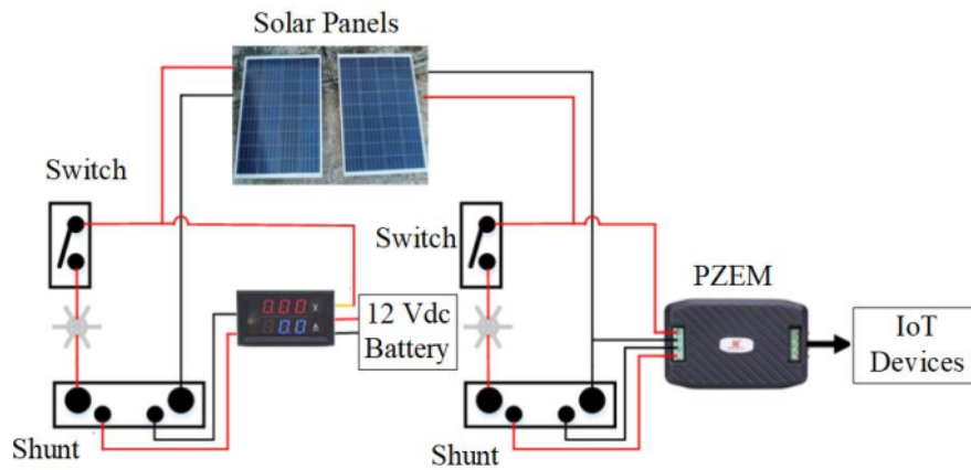
Figure 5. The wiring diagram of the PV system
