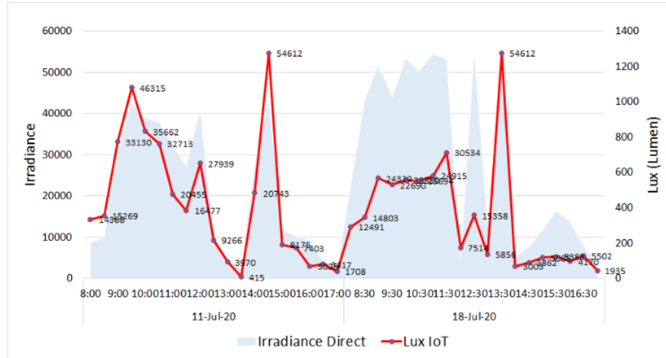
Figure 8. The comparison between Lux and Irradiance measurement
