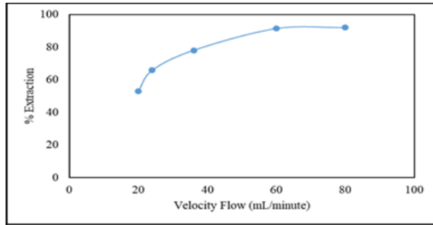
Fig. 2. Effect of Speed of Feed Phase Flow
