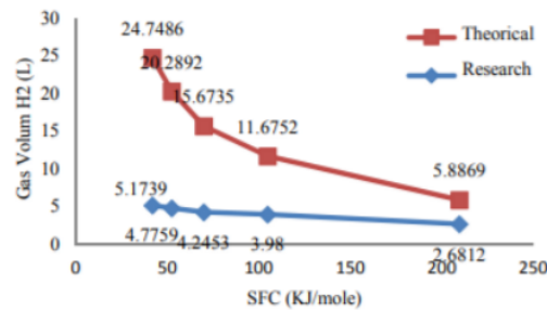
Fig. 4. The Relationship of SFC (Specific Fuel Consume) to the Volume of Hydrogen Gas produced by Theory and Research
