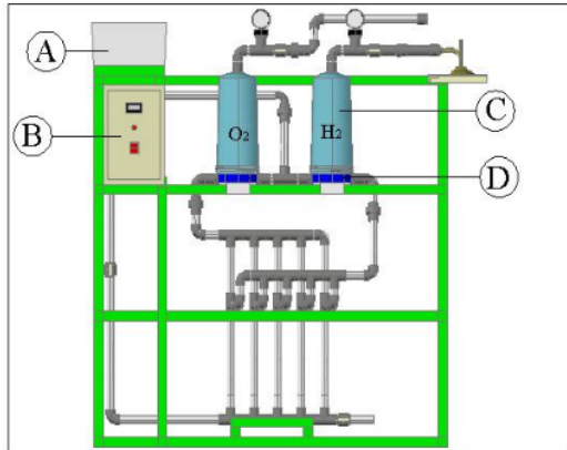
Fig. 1. Water electrolyzer design
