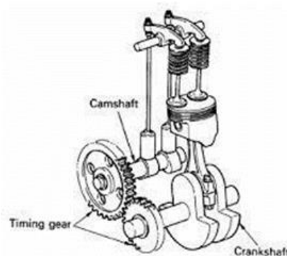
Gambar 2.4 Timing Gear (Ilmuotomotiv, 2022)
