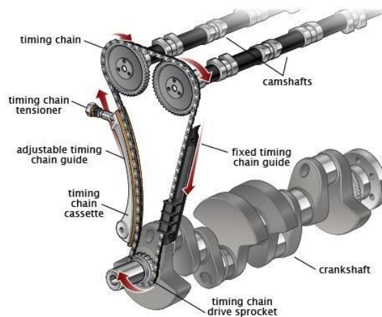
Gambar 2.5 Timing Chain (Repairpal, 2022)
