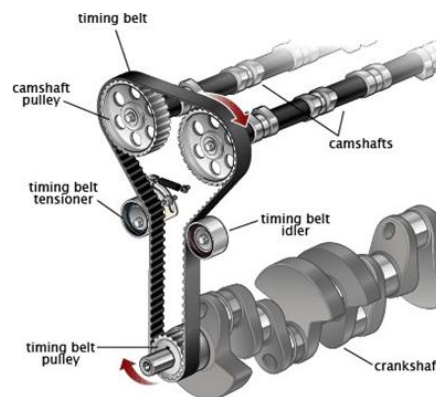
Gambar 2.3 Timing Belt (Bacabrosur, 2022)
