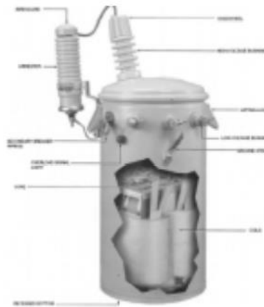
Gambar 2. 24 Transformator CSP ( Completely Self Protected )
