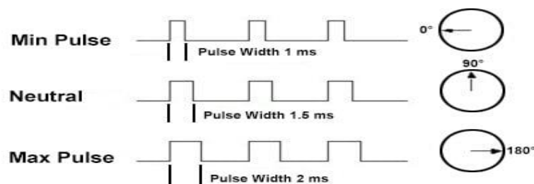
Gambar 2.10 Pulse Wide Modulation Servo
