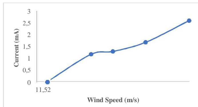
Figure 5. Current output of the wind turbine
