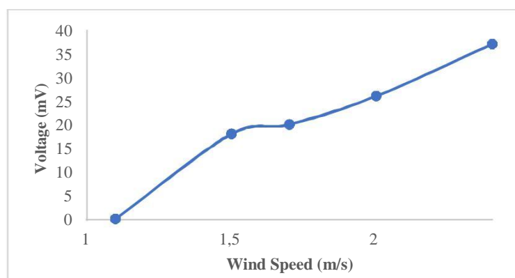
Figure 4. Voltage output of the wind turbine
