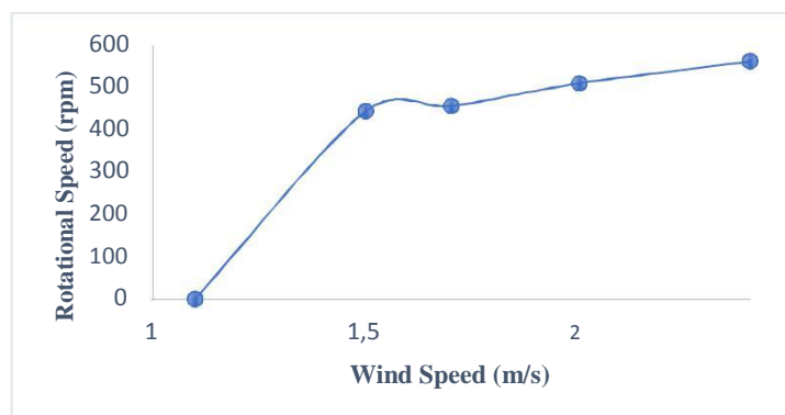
Figure 3. Rotational speed output of the wind turbine
