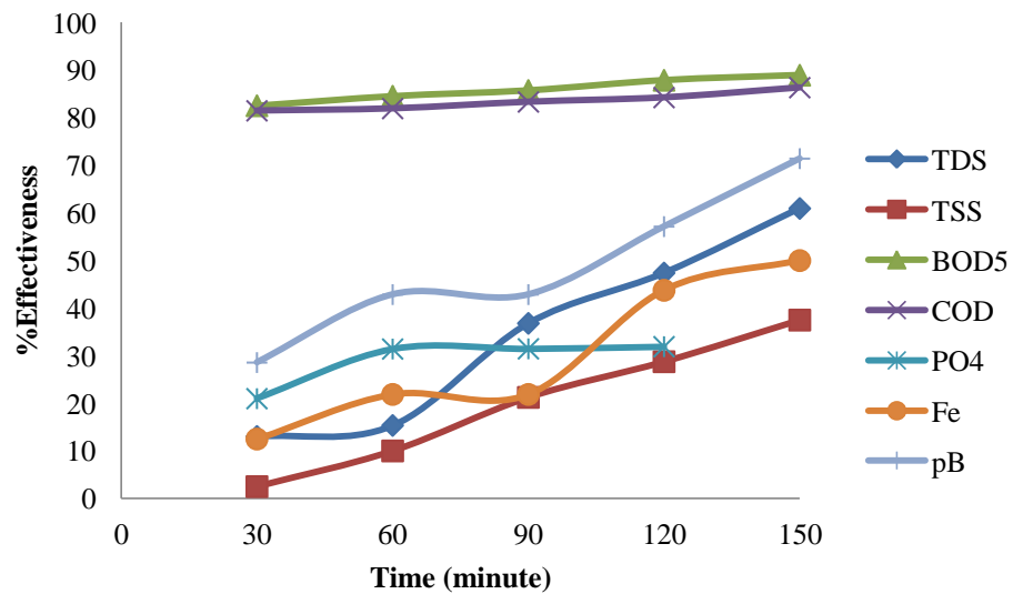
Figure 2. Effectiveness of the Electrocoagulation Method Against Time at a Voltage of 6 V Using Aluminum Electrode
