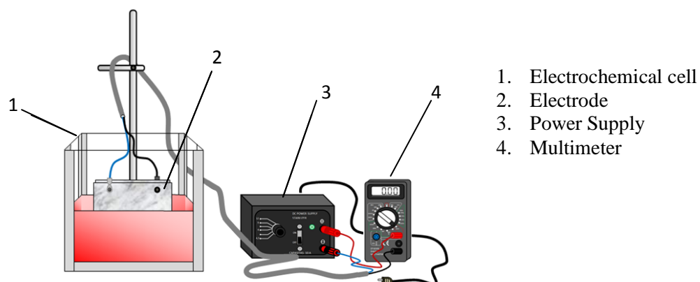
Figure 1. Batch electrocoagulation system
