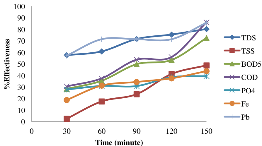
Figure 6. Effectiveness of the Electrocoagulation Method Against Time at a Voltage of 9V Using Stainless Steel Electrode
