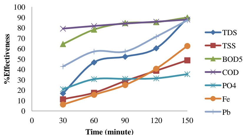
Figure 4. Effectiveness of the Electrocoagulation Method Against Time at a Voltage of 12 Volts Using Aluminum Electrode
