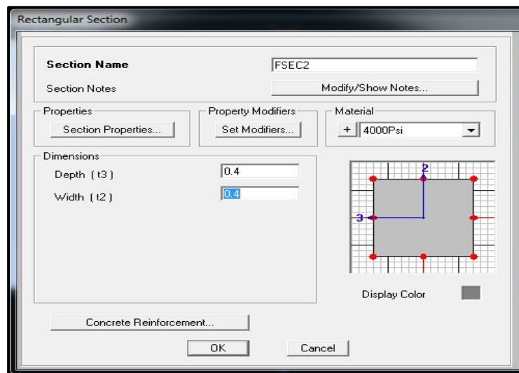
Gambar 2.14 Jendela Rectangular Section
