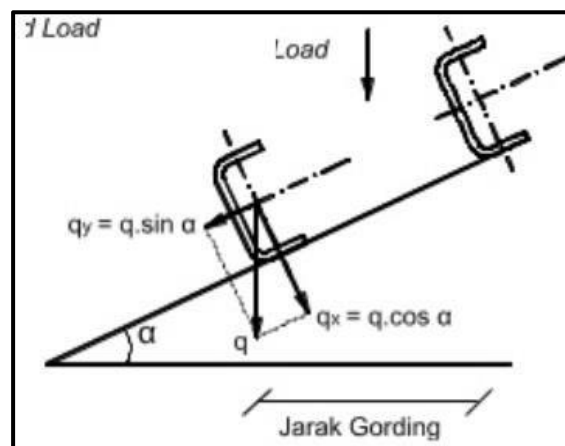
Gambar 2. 1 Uraian Beban Gording
