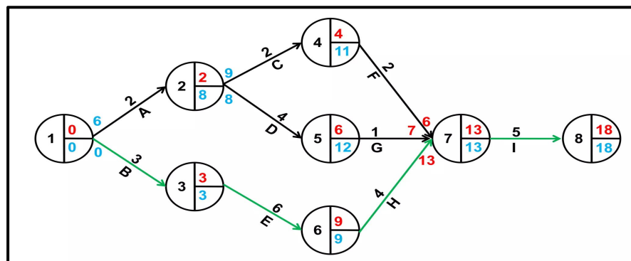
Gambar 2. 20 Diagram NWP
