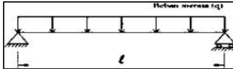
Gambar 2. 2 Beban Merata Gording
