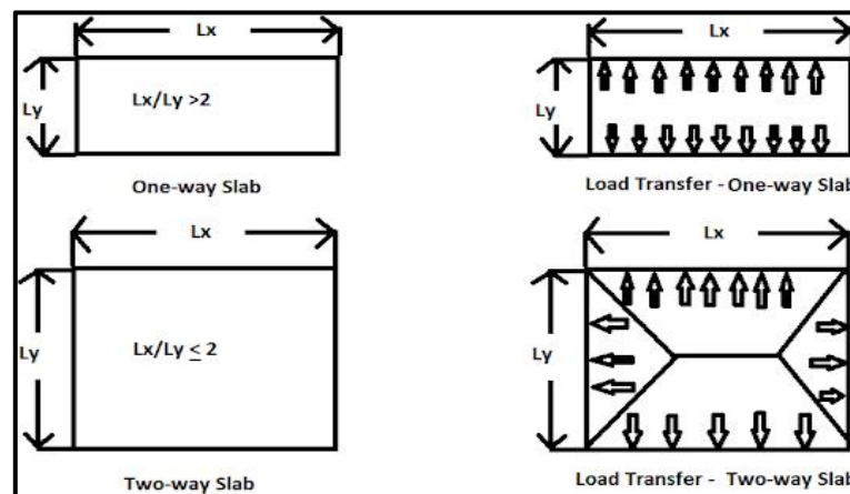
Gambar 2. 5 Diagram Transfer Pembebanan
