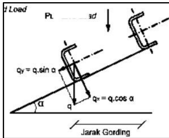
Gambar 2. 3 Uraian Beban Gording
