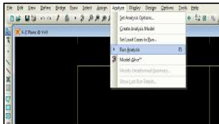
Gambar 2.18 Run Analisis
