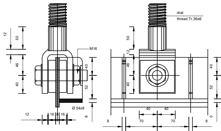
DETAIL I
