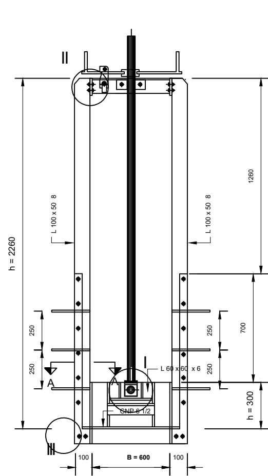
TAMPAK DEPAN FRONT VIEW
