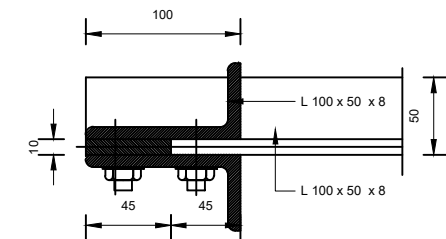
DETAIL II
