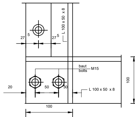
DETAIL III
