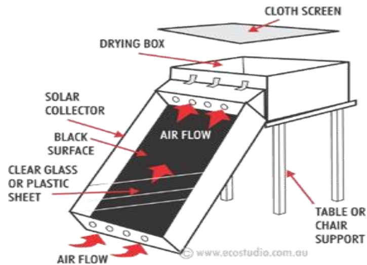
Gambar 2.2 Solar Dryer ( Docplayer, 2019 )
