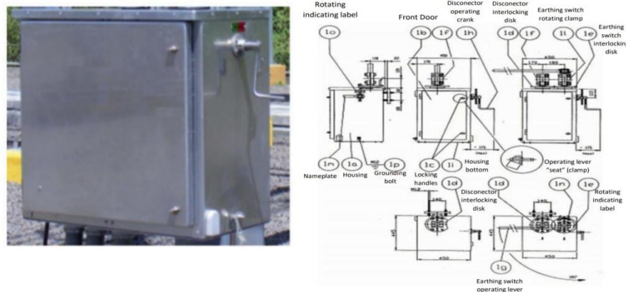
Gambar 2.5 Lemari Mekanik
