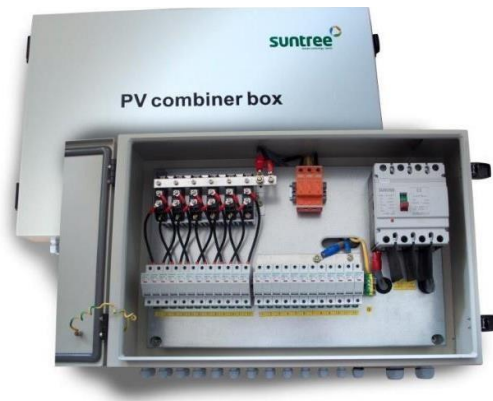
Gambar 2 23 combiner box
