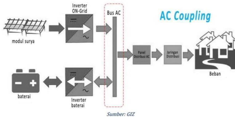
Gambar 2 4 Diagram Sistem PLTS Off-Grid tipe AC Coupling
