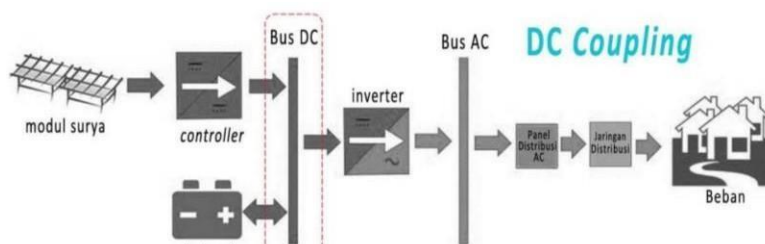
Gambar 2 5 Diagram Sistem PLTS Off-Grid tipe DC Coupling
